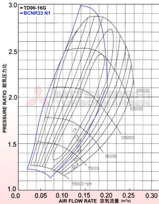
COMPRESSOR MAP
