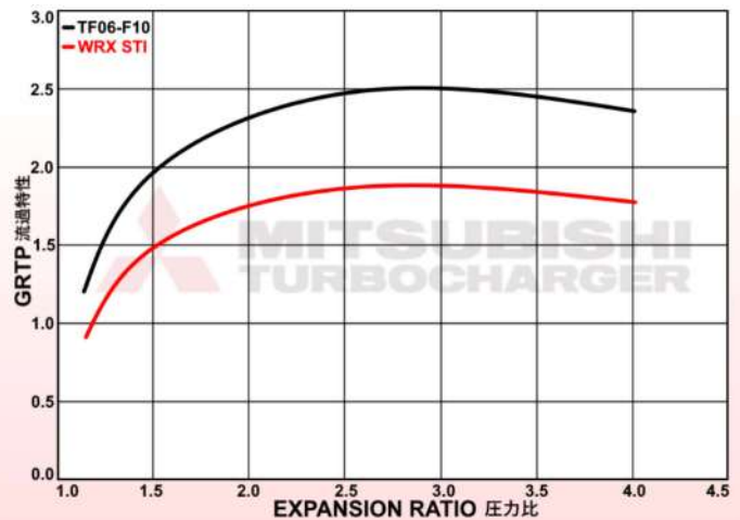
TURBINE MAP
