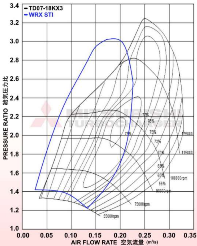
COMPRESSOR MAP
